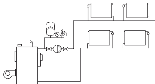
Fig. 2 One-pipe heating system
