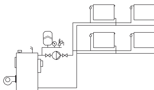
Fig. 3 Two-pipe heating system
