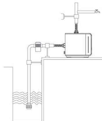
Fig. 4 Suction from well or tank
