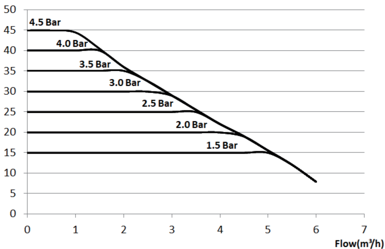
Fig.6 Performance curves
