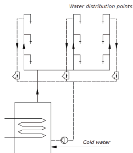
Fig.3 Functional drawing of multi-circuit hot water recirculation
