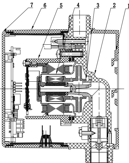
Fig. 7 Sectional drawing
