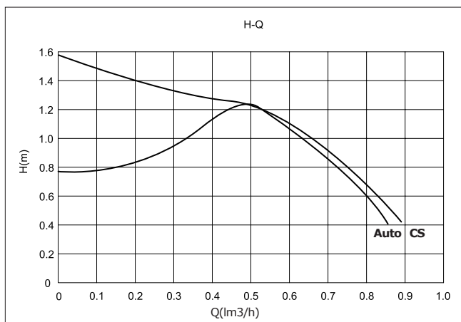
Fig.4 Performance curve
