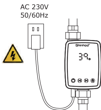
Fig.6 Wiring Diagram
