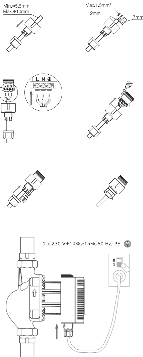
Fig. 36 Electrical connection
